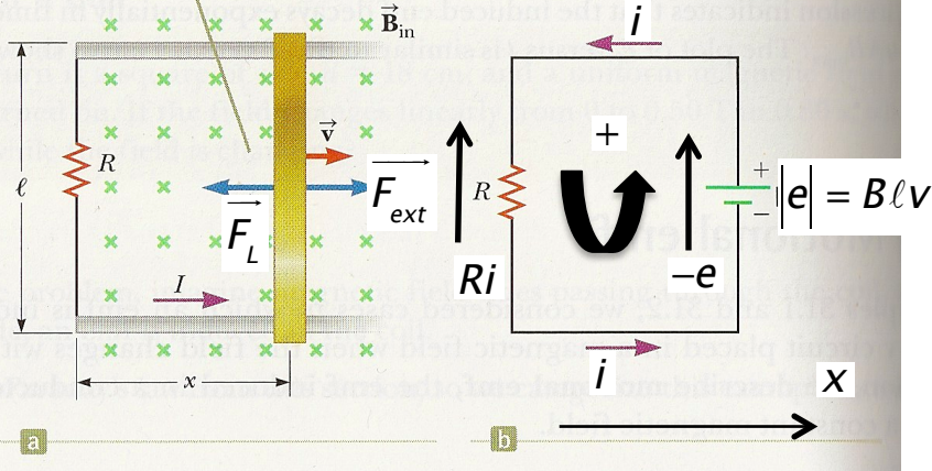
Figure 31.8 (a) A conducting bar sliding with a velocity \vec{v} along two conducting rails under the action of an applied force \vec{F}_{app} . (b) The equivalent circuit diagram for the setup shown in (a).
