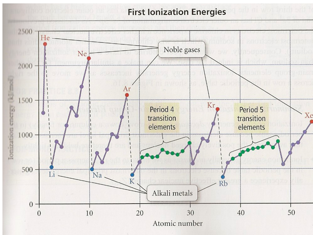
◀ FIGURE 8.15 First Ionization Energy versus Atomic Number for the Elements through Xenon Ionization starts at a minimum with each alkali metal and rises to a peak with each noble gas.
