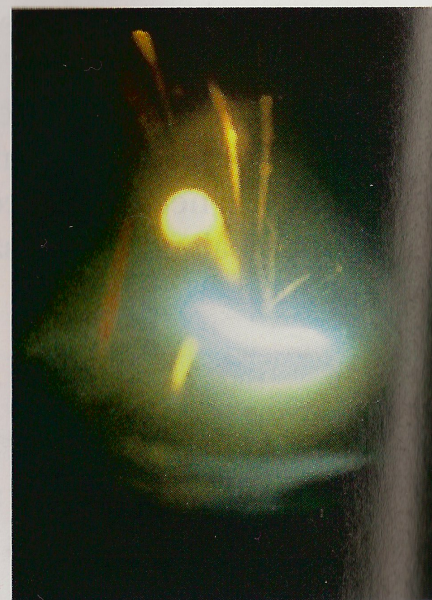
(c) Reaction of phosphorus and oxygen to give tetraphosphorus decaoxide, \text{P}_4\text{O}_{10} .
