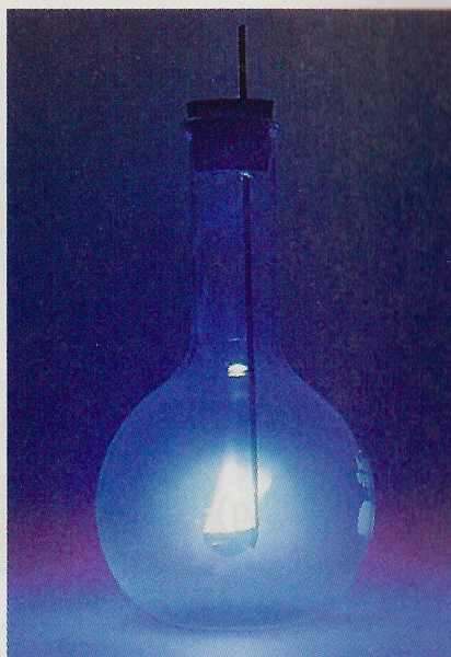
(b) Reaction of sulfur (in the spoon) with oxygen.
