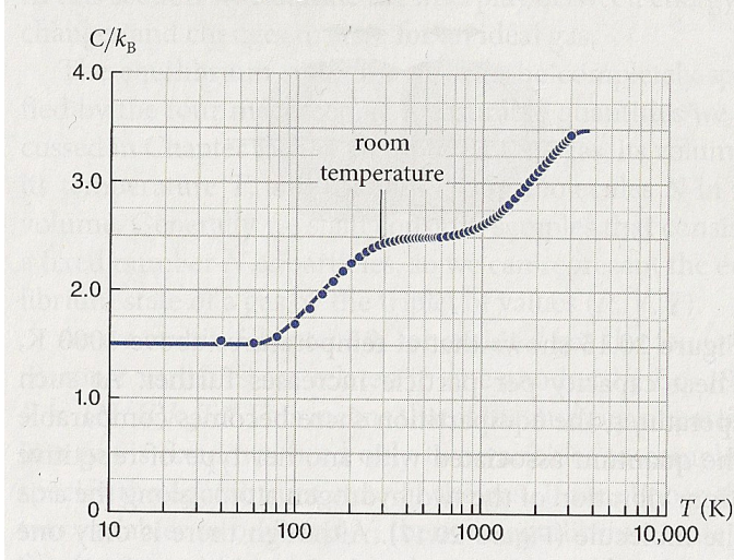
Figure 20.15 Temperature dependence of the heat capacity per particle C in units of k_B for hydrogen gas molecules.
