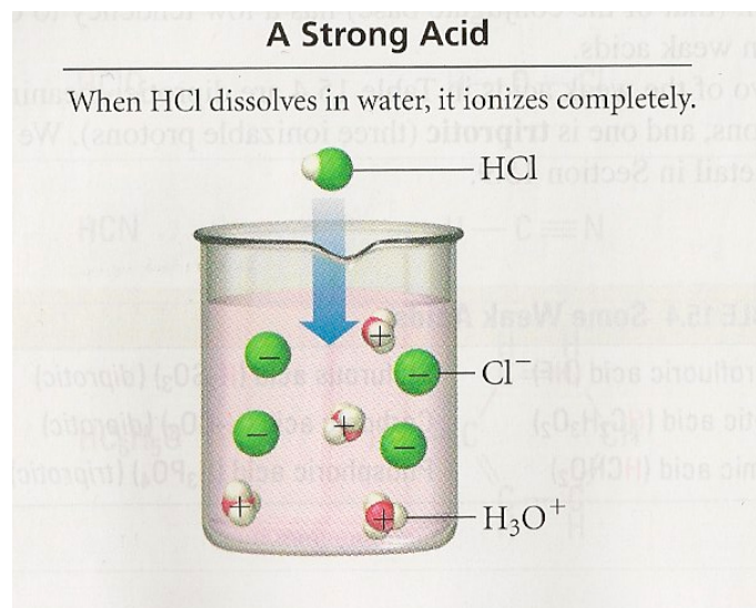
◀ FIGURE 15.4 Ionization of a Strong Acid When HCl dissolves in water, it completely ionizes to form \text{H}_3\text{O}^+ and \text{Cl}^- . The solution contains virtually no intact HCl.
