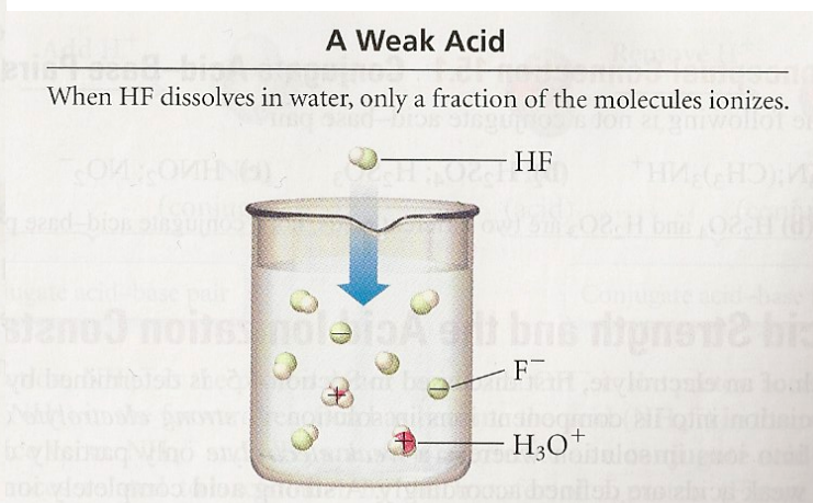
▶ FIGURE 15.5 Ionization of a Weak Acid When HF dissolves in water, only a fraction of the dissolved molecules ionize to form \text{H}_3\text{O}^+ and \text{F}^- . The solution contains many intact HF molecules.
