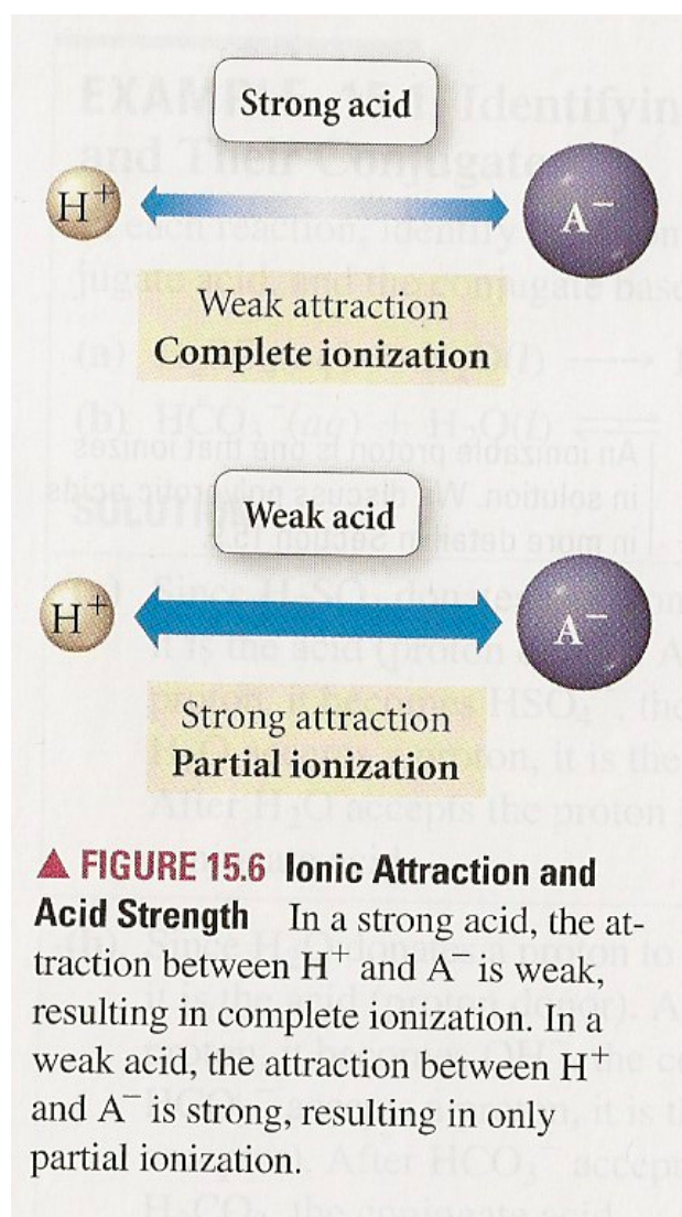
▶ FIGURE 15.5 Ionization of a Weak Acid When HF dissolves in water, only a fraction of the dissolved molecules ionize to form \text{H}_3\text{O}^+ and \text{F}^- . The solution contains many intact HF molecules.
