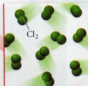
▲ FIGURE 4.21 Oxidation-Reduction without Oxygen When sodium reacts with chlorine, electrons are transferred from the sodium to the chlorine, resulting in the formation of sodium chloride. In this redox reaction, sodium is oxidized and chlorine is reduced.
